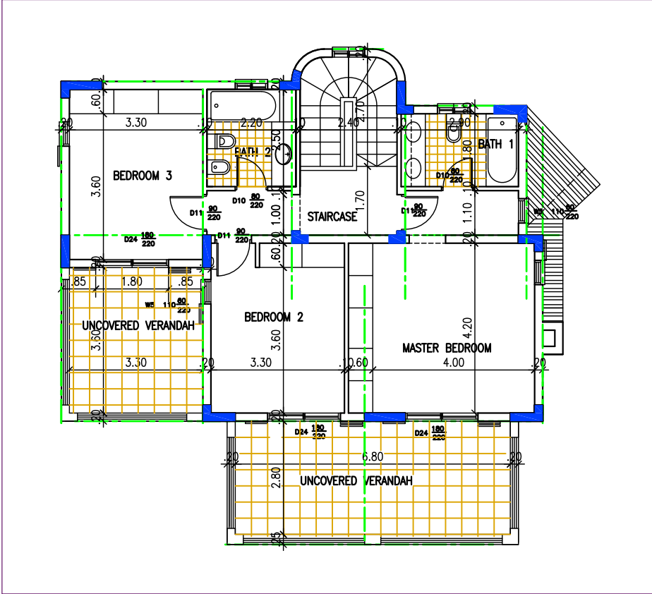
PRELIMINARY FIRST FLOOR PLAN
