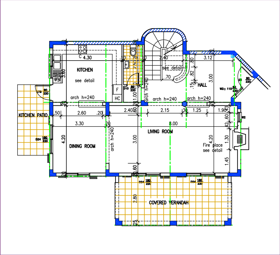
PRELIMINARY GROUND FLOOR PLAN
